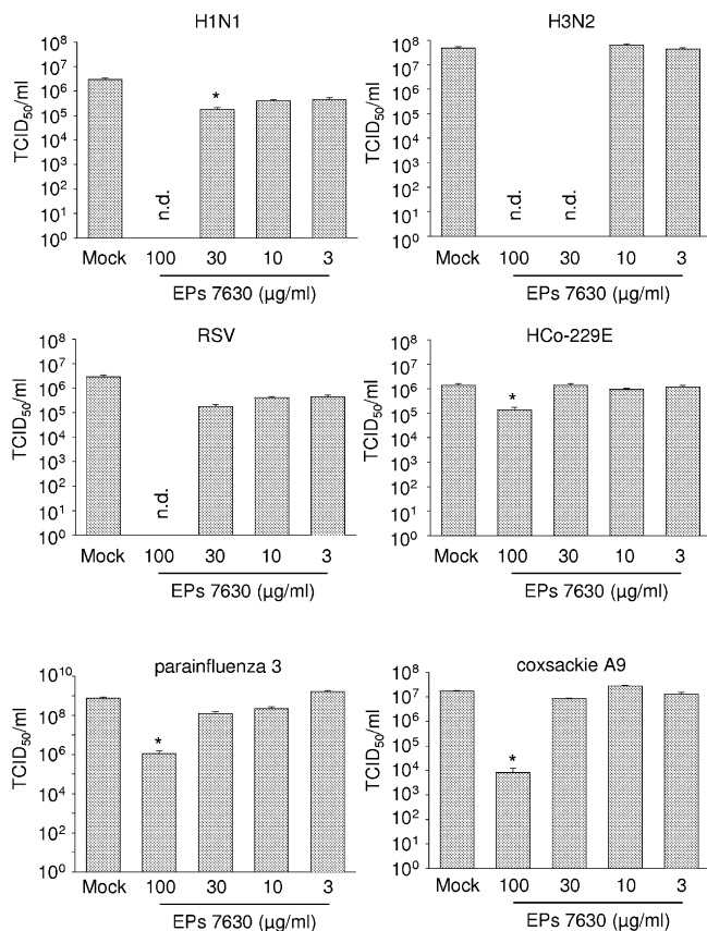
Fig. 1. Influence of EPs ® 7630 on infectious virus titres indicated as 50% tissue culture infectious dose (TCID 50 /ml). EPs ® 7630 was continuously present in cell culture media beginning with a 1 h pre-incubation period. Cells were infected with the respective viruses in the absence (Mock) or presence of EPs ® 7630 at the following MOIs: influenza A virus H1N1, 0.005 (titres were determined 24 h post infection, cell line MDCK); influenza A virus H3N2, 0.005 (24 h, MDCK); coxsackie virus A9 (coxsackie A9), MOI 0.005 (24 h, human foreskin fibroblasts); parainfluenza virus type 3 (parainfluenza 3), 0.01 (72 h, LLC-MK2); respiratory syncytial virus (RSV), 0.01 (72 h, Vero); human coronavirus strain 229E (HCoV-229E), 0.01 (72 h, Caco-2). * P < 0.05 relative to Mock (as determined by ANOVA with subsequent Student–Newman–Keuls test); n.d. = not detectable.
